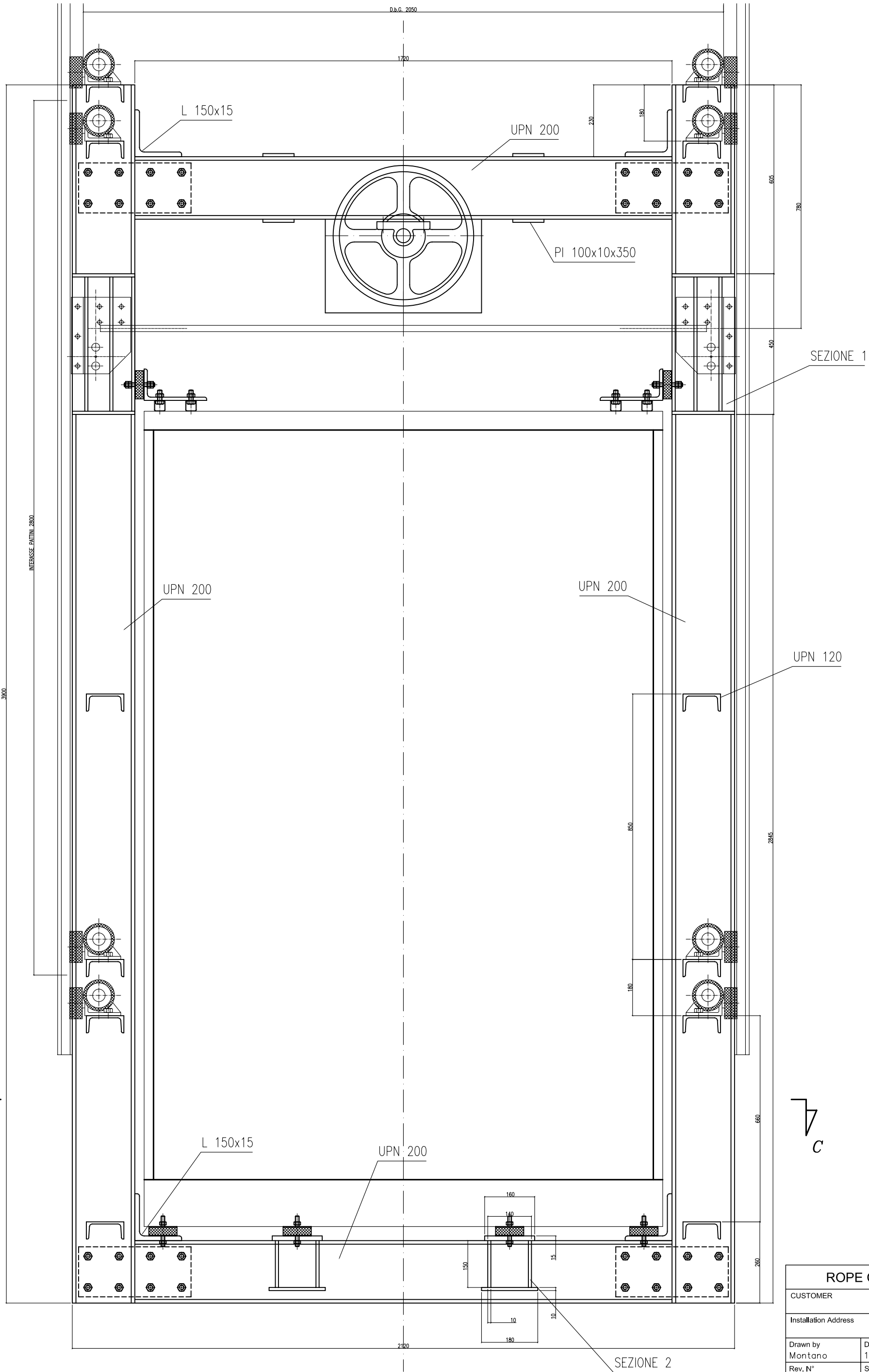
CAR FRAME - FRONT VIEW Scale 1:12
